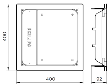
BBP500 LED84/125/140 PSU & PSD
