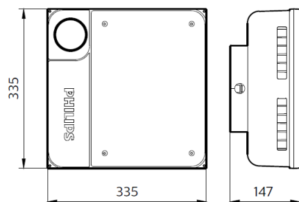
BCP500 LED180 PSU & PSD
