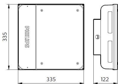
BCP500 LED84/125/140 PSU & PSD
